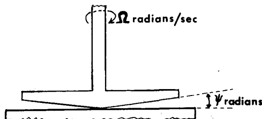
FIG. 6-18. Basic configuration of the cone and plate viscometer.
