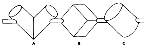
FIG. 1-11. Three types of tumbling mixers shown mounted on a common shaft: A, twin-shell; B, cubic; C, cylindric. In operation, the asymmetric geometry results in a sideways movement of material in addition to the tumbling action of the mixers. Of the three types, the twin-shell is the most popular.
