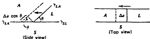
FIG. 5-30. Schematic of derivation of Young equation based on the change in free energy caused by an increase in the area of a solid, \Delta a , which is wetted by a liquid. (From Rosen, M. J.: Surfactants and Interfacial Phenomena . John Wiley and Sons, New York, 1978, p. 178.)
