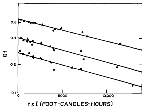
FIG. 26-31. Plots of \theta_t vs. the product of time and intensity. Key: ●, 11 footcandles; ▲, 50 footcandles; ■, 80 footcandles; ▼, 655 footcandles. Top line, 0.06% dye; middle line, 0.03%; bottom line, 0.015% dye. (From Everhard, M. E., and Goodhardt, F. W.: J. Pharm. Sci. , 52:281, 1963.)
