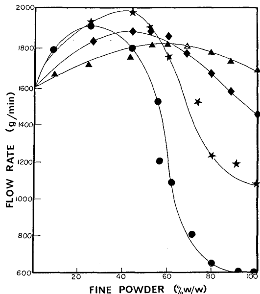
FIG. 4-3. Effect of fines on the rate of flow of mixtures of coarse granules (0.561 mm) as a function of increasing amounts of fines: (▲) 0.158 mm; (◆) 0.09 mm; (★) 0.059 mm; (●) 0.048 mm. (From Jones. 1 Reproduced with permission of the copyright owner.)
