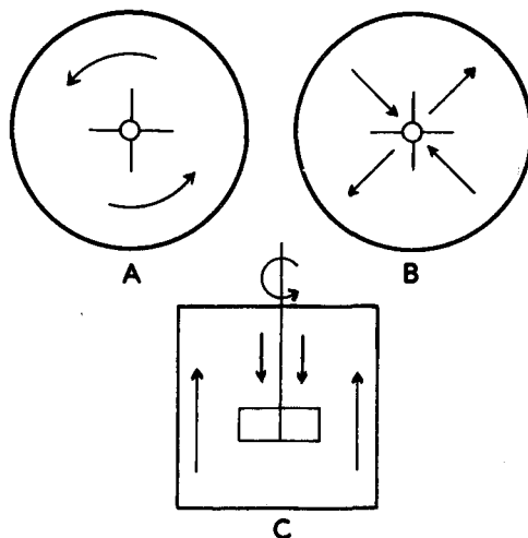
FIG. 1-2. A and B, Diagrammatic representation of cylindric tanks in which tangential and radial flow occur, respectively. C, Side view of a similar tank in which axial flow occurs. These diagrams represent systems in which only one type of flow occurs, in contrast to the usual situation in which two or more of these flow patterns occur simultaneously.
