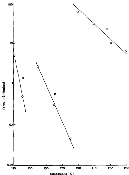
FIG. 21-2. Z value plots of log D versus temperature. Key—A: Z = 10^\circ\text{C} for B. stearothermophilus spores exposed to steam sterilization. B: Z = 22^\circ\text{C} for B. subtilis var niger spores exposed to dry heat sterilization. C: Z = 54^\circ\text{C} for E. coli endotoxin exposed to dry heat sterilization.
