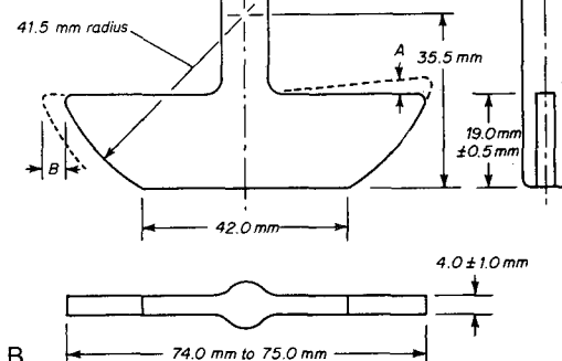
FIG. 11-4. A, USP dissolution apparatus 1. B, USP dissolution apparatus 2. (Reproduced from the Third Supplement to USP XX-NF XV, © 1982, USP Convention, pages 310 and 311. Permission granted.)
