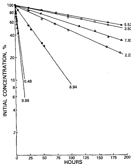
FIG. 26-5. Observed pseudo-first-order plots for the degradation of I at various pH values, 25^\circ , and \mu = 0.5 . Key: \square , pH 5.52; \circ , pH 3.93; \blacktriangle , pH 7.93; \diamond , pH 2.23; \blacksquare , pH 8.94; \bullet , pH 0.48; \triangle , pH 9.89. (From Berge, S. M., et al.: J. Pharm. Sci. , 72:59, 1983. Reproduced with permission of the copyright owner, the American Pharmaceutical Association.)
