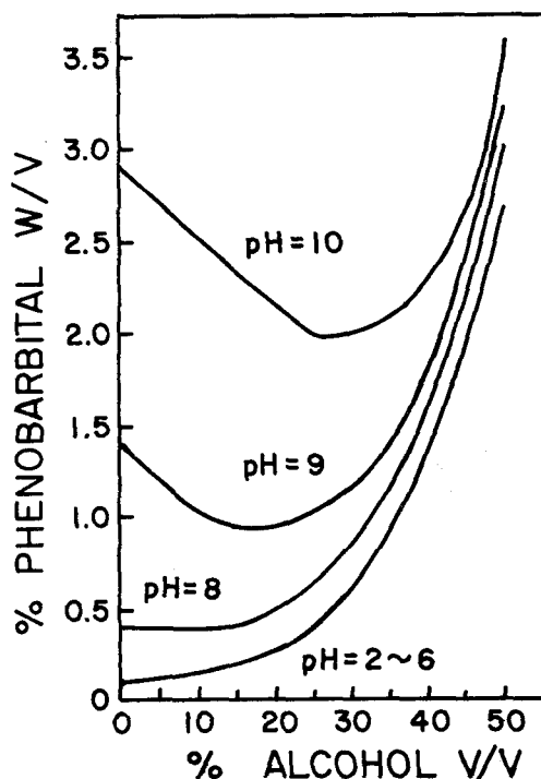
FIG. 15-4. Interdependence of pH and alcohol concentration on the solubility of phenobarbital. (From Lin, K.S., Anschel, J., and Swartz, C.J.: Bull. Parenteral Drug Assoc., 25:44, 1971.)
