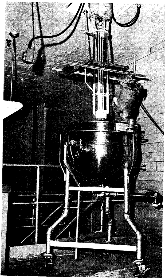
FIG. 18-6. The high shear Homo-Mixer is attached to an electrically driven lift mechanism for raising or lowering it into the jacketed kettle used for dispersing solids in liquids. (Permission of Ciba-Geigy Corp.)
