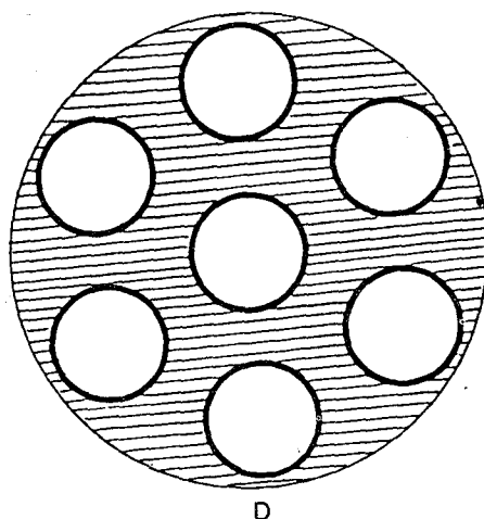
FIG. 4-12. Stages in the development of moist granules as the proportion of liquid is increased: pendular (A), funicular (B), capillary (C), and droplet (D). (After Newitt and Conway-Jones. 12 )
