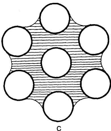
FIG. 4-12. Stages in the development of moist granules as the proportion of liquid is increased: pendular (A), funicular (B), capillary (C), and droplet (D). (After Newitt and Conway-Jones. 12 )
