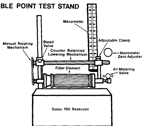
FIG. 7-12. Apparatus for performing the visible bubble test for cartridge filters. 26 (From Field Experience in Testing Membrane Filter Integrity by the Forward Flow Test Methods , Bulletin AB710-1-75. Pall Corporation, NY.)
