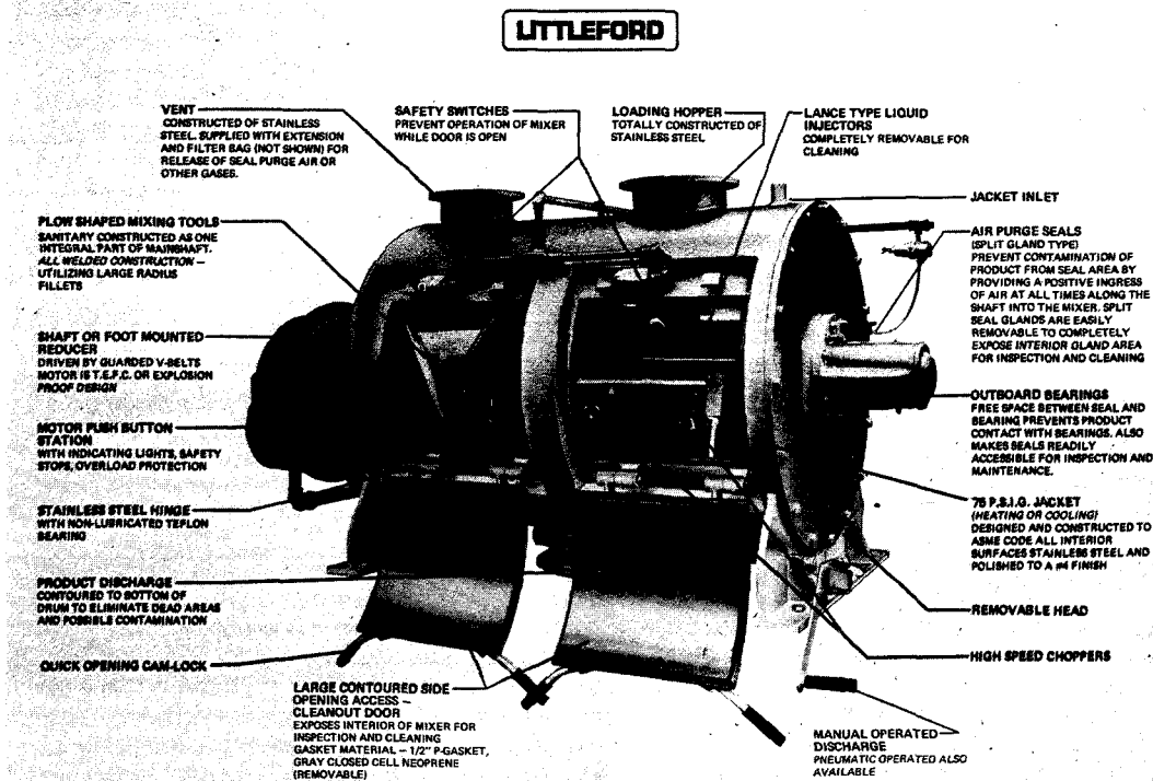
FIG. 11-14. The Littleford Lodge mixer. (Courtesy of Littleford Brothers, Florence, KY.)
