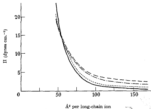
FIG. 5-15. Film-pressure/area curves of octadecyltrimethyl ammonium cation in sodium chloride solutions of various concentration. Key: —, 0.033 M sodium chloride; —•—, 0.1 M sodium chloride; ····, 0.5 M sodium chloride; — — —, 2 M sodium chloride. (From Davies, J. T.: Proc. R. Soc. Lond. , A208:224, 1951.)
