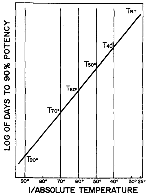
FIG. 26-10. Plot of t_{10\%} values vs. absolute temperature -1 (From Blythe, R. H.: Product Formulation and Stability Prediction . Presented at the Production Section of the Canadian Pharm. Mfgs. Assoc., April 1957.)
