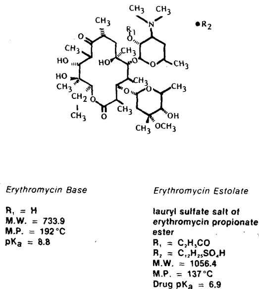
FIG. 8-3. Structures of erythromycin and its estolate pro-drug.
