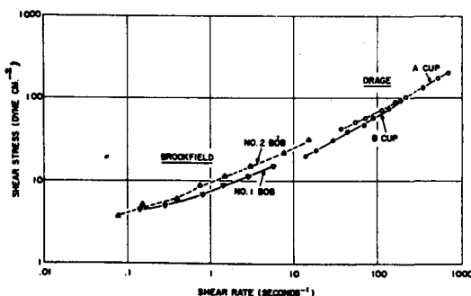
FIG. 6-17. Type of overlapping rheograms obtained with different cup and bob combinations, using equations without correction. (From Wood, J. H., Catacalos, G., and Lieberman, S. V. (J. Pharm. Sci. 52:296, 1963. Reproduced with permission of the copyright owner, the American Pharmaceutical Association.)
