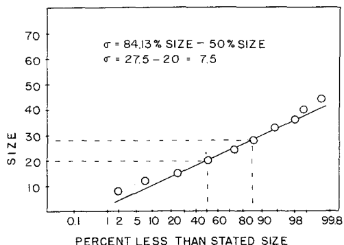
FIG. 2-3. Arithmetic-probability plot of data in Table 2-2.
