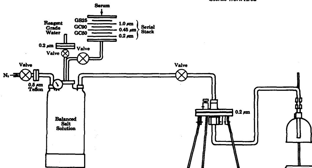
FIG. 7-9. Schematic representation of operational sequence.
