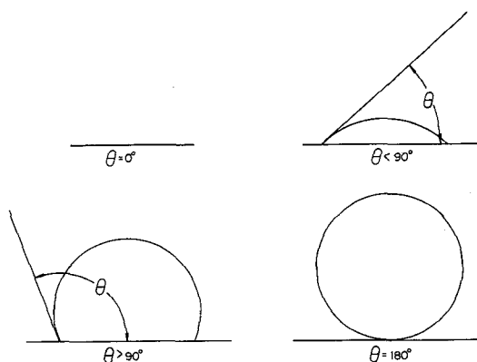
FIG. 5-29. The use of the contact angle, \theta , to characterize the wetting of a solid by a liquid.
