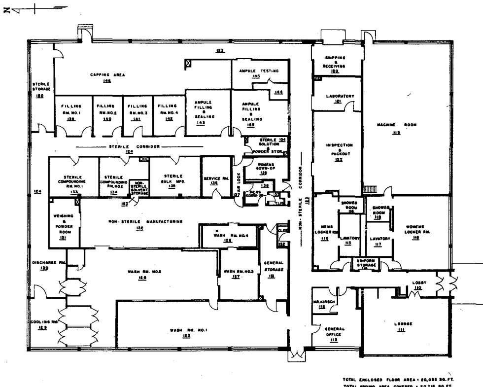
FIG. 22-4. Floor plans for industrial sterile products production area. (Courtesy of Schering Corp.)
