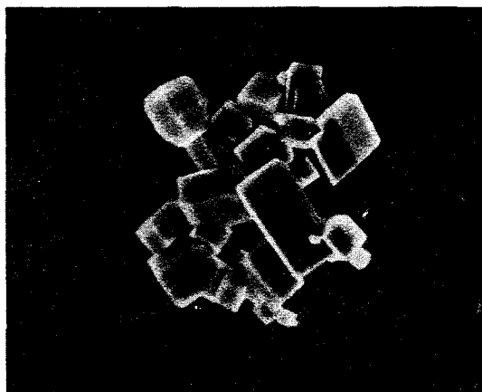
FIG. 26-42. Scanning electron micrographs of barium sulfate crystals isolated from procaine hydrochloride (A) and atropine sulfate (B) (1000 \times , 20 kv). (From Boddapati, S., Butler, D. L., Im, S., and DeLuca, P. P.: J. Pharm. Sci. , 69:608, 1980. Reproduced with permission of the copyright owner, the American Pharmaceutical Association.)
